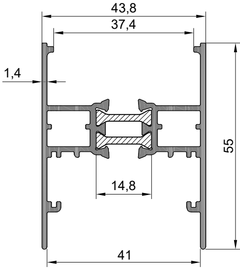
ASM41T-11 1,009kg/mt
