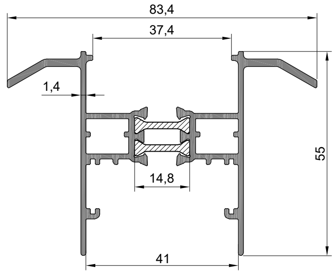
ASM41T-14 1,175 kg/mt
