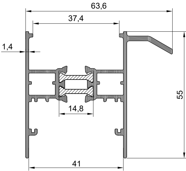
ASM41T-13 1,129 kg/mt
