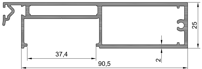
ASM41T-43 1,359 kg/mt
