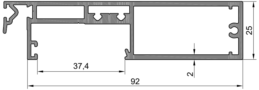
ASM41T-44 1,524 kg/mt
