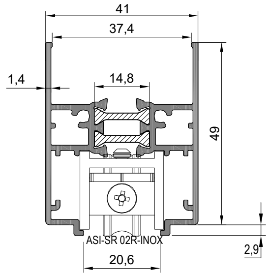
ASM41T-12 1,008 kg/mt
