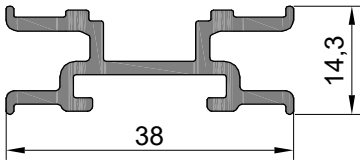
ASM41T-62 0,440 kg/mt
