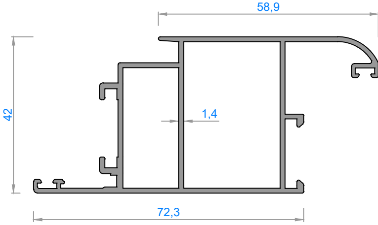
2943 - 1,105 kg/m
