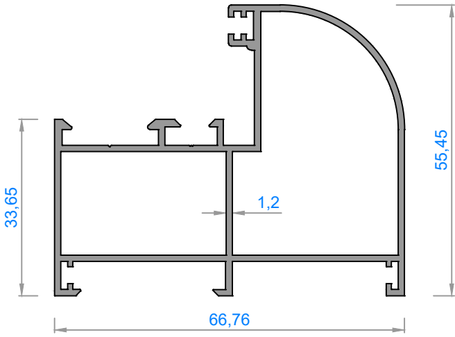
1326 - 1,000 kg/m
