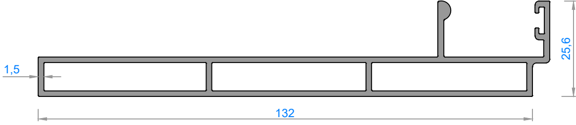
5987 - 1,390 kg/m
