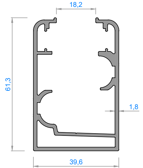
4910 - 1,210 kg/m
