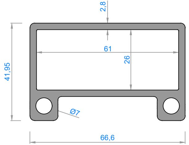
3968 - 1,884 kg/m
