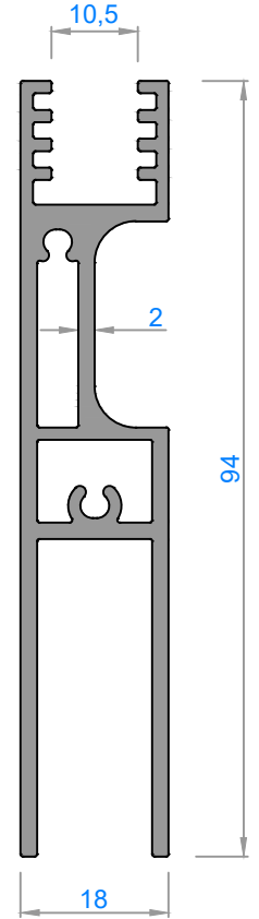
4452 - 1,368 kg/m
