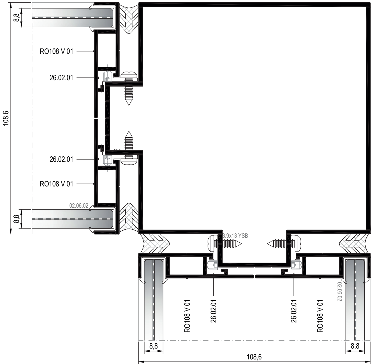
34 DETAYI DETAIL
